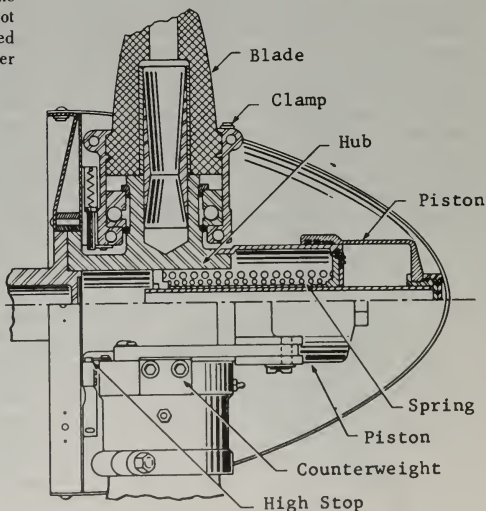
FIGURE 7-14. Constant-speed feathering.
